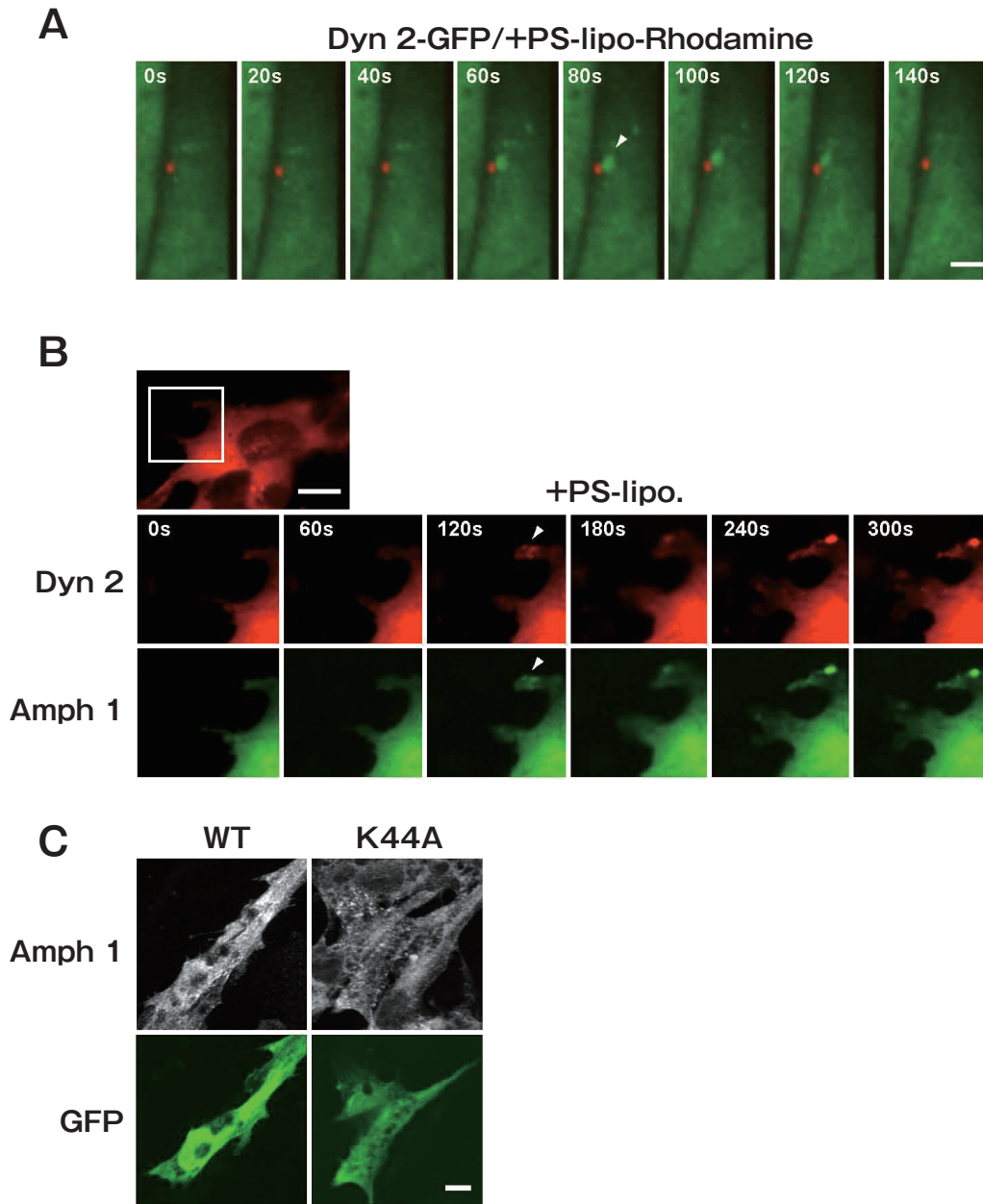
Fig. 3 Dynamin 2 may cooperate with amphiphysin 1 in PS-dependent phagocytosis. A , Dual-live imaging of dynamin 2-GFP (green) and rhodamine-labeled PS-liposome (red) in Ser-W3 cells. Cells expressing dynamin 2-GFP were stimulated with rhodamine-PS-liposomes, and images were taken every 20sec. Note that dynamin 2-GFP transiently accumulated at the phagocytic site. Bar: 5 \mu m. B , Dual-live imaging of dynamin 2-mCherry (red) and GFP-amphiphysin 1 (green) in PS-stimulated Ser-W3 cells. Images of area surrounded by a rectangle in the top panel were taken every 60sec. Both GFP and mCherry fluorescence simultaneously appear at ruffles (arrowheads). The scale bar represents 10 \mu m in upper panels, 5 \mu m in lower panels; C , Mutant dynamin 2 (K44A) induces mis-localization of amphiphysin 1 in PS-stimulated Sertoli cells. Wild-type or mutant dynamin were co-transfected with EGFP (dynamin : EGFP = 10 : 1 in cDNA ratio) in primary cultured rat Sertoli cells. The cells were stimulated with PS-liposomes, as described in Fig. 1A, and stained for amphiphysin 1. Note that immuno-reactivity for amphiphysin1 is represented as large dots in dynamin K44A expressing cells (upper right), which can be identified by GFP expression (lower right). Bar: 10 \mu m.
